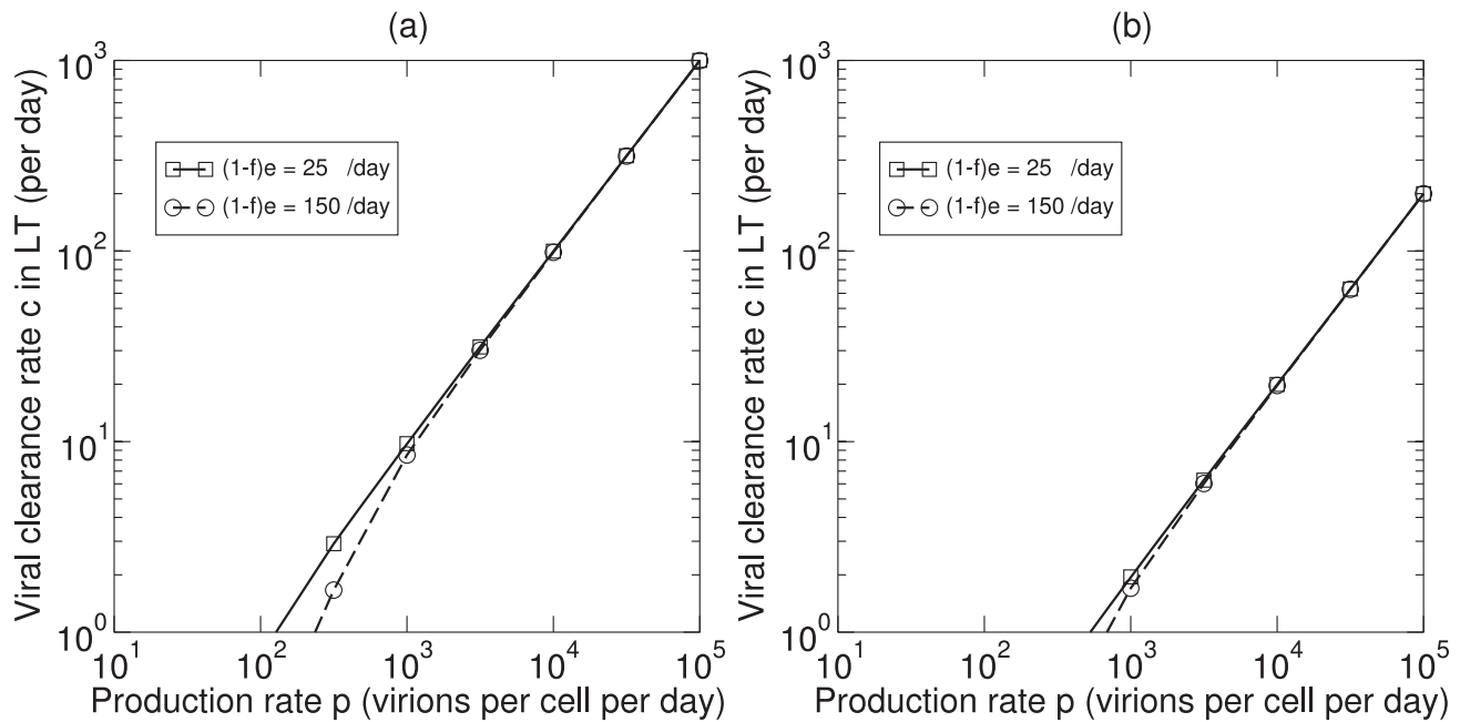
Figure 1. Viral clearance in the lymphoid tissue, c , as a function of the production rate p , given by Eq. (14), for a typical patient with I = 10^8 cells, V_P = 10^8 , V_L = V_F + V_B = 10^{11} particles, and the indicated clearance rates via the blood, (1-f)e . In (a) 90% of the virus in lymphoid tissue is associated with FDCs, i.e., V_F = 10^{10} , and in (b) this is 50%, i.e., V_F = 5 \times 10^{10} . doi:10.1371/journal.pcbi.1000906.g001
