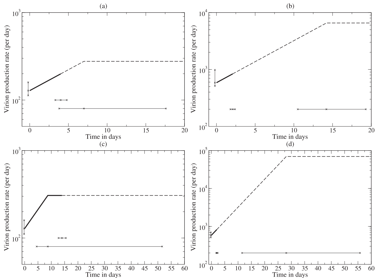
Figure 3. Viral production rates in the lymphoid tissue estimated by Reilly et al. [23] for resting (panels a,c) and activated cells (b,d) respectively. The top row of the Figure (Panels a,b) is the result when the mean of the prior distribution of the half-life resting cells is 4 days (and that of activated cells is 1.5 days). In the bottom row (c,d) the mean of the prior distribution of the half-life resting cells is 14 days (and that of activated cells remains 1.5 days). The median total production rate per cell is computed by integrating these curves up to the half-life of the cell (as indicated by the heavy lines) and amounts to 1479 and 1395 virions per activated cell and 644 and 3405 per resting cell (see the text). The horizontal and vertical lines marked by crosses denote the mean value with 95% credible intervals for the production rate at time zero, the half-life of the cell, and the saturation time of the production function [23]. doi:10.1371/journal.pcbi.1000906.g003
