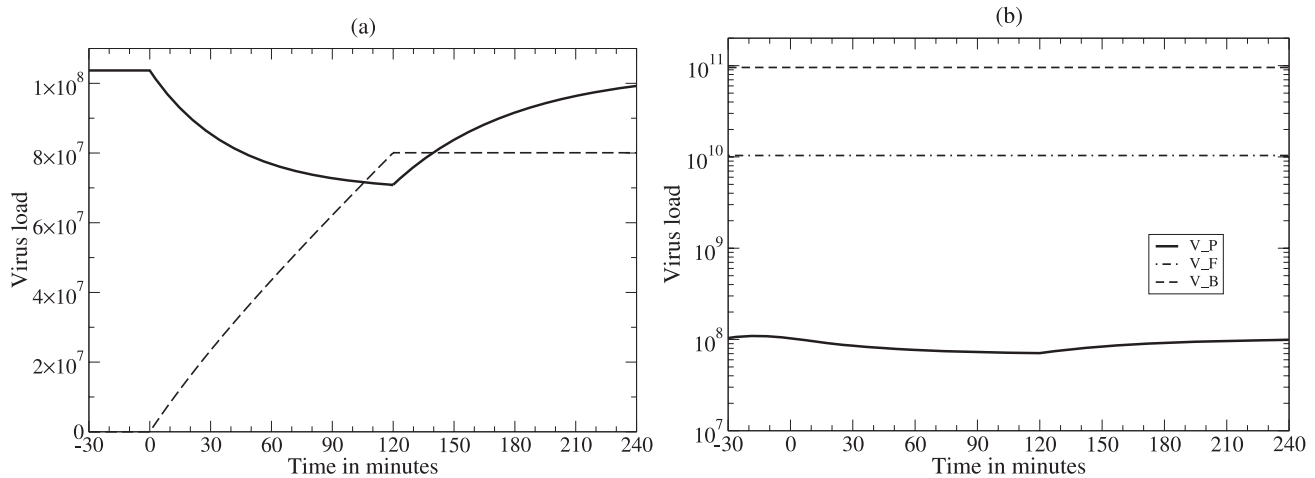
Figure 2. Plasma apheresis for 2 hrs simulated in the model for a patient with V_P \approx 10^8 , V_F \approx 10^{10} and V_B \approx 10^{11} virus particles in the total body. The solid line is the plasma viral load ( V_P ). The discontinuities reflect the time period of plasma apheresis which starts at time zero and continues for two hours (during this period we set \epsilon = 12 \text{ d}^{-1} ; otherwise \epsilon = 0 ). The dashed line in (a) is the total amount of virus removed ( V_R ), i.e., the solution of dV_R/dt = \epsilon V_P . The dashed line in (b) is virus bound to FDCs ( V_B ), and the dash-dotted line in (b) is free virus in lymphoid tissue ( V_F ). Parameters: \phi = 1 , F = 10^{11} , c = 48 \text{ d}^{-1} , e = 24 \text{ d}^{-1} , \epsilon = 12 \text{ d}^{-1} , f = 0.1 , i = 0.24 \text{ d}^{-1} , k_1 = 8.64 \times 10^{-6} \text{ d}^{-1} , k_2 = 8640 \text{ d}^{-1} ( 0.1 \text{ s}^{-1} ), n = 1 , pI = 5 \times 10^{11} particles \text{d}^{-1} . The results in this Figure are independent of the parameter c_0 because we are only solving for V_P , V_F , and V_B (see Eqs. 7–9). doi:10.1371/journal.pcbi.1000906.g002
