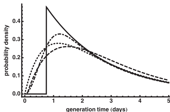
FIG. A2. Generation time distributions resulting from different viral production kernels. Assuming that viral production rates increase with the age of an infected cell influences the shape of the generation time distribution. The standard model (model 1) follows an exponentially distributed generation time after the intracellular delay (solid line). Increases in viral production rates with the age of infected cells result in shorter intracellular delays and a smoothing of the generation time distribution. Dashed line, linearly increasing viral production rate (model 2); dotted line, exponentially increasing viral production rate (model 3a); dashed-dotted line, sigmoidally increasing viral production rate (model 4). Note that the means for all four distributions are roughly the same (Table 2).
